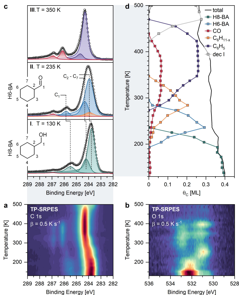
Figure 3. SRPES results for H8-BA on Pt(111). (a and b) Color-coded density plots of the C 1s ( h\nu = 380 eV) and O 1s ( h\nu = 650 eV) temperature-programmed XPS experiments ( \beta = 0.5 K ^{-1} ); initial surface coverages after H8-BA adsorption at 130 K were \sim 0.40 and 0.38 C-ML, respectively. (c) Selected, individual XP spectra from the C 1s experiment with the applied fit model. (d) Corresponding quantitative analysis of the C 1s experiment, including the legend, which explains the color code of the fit model.
